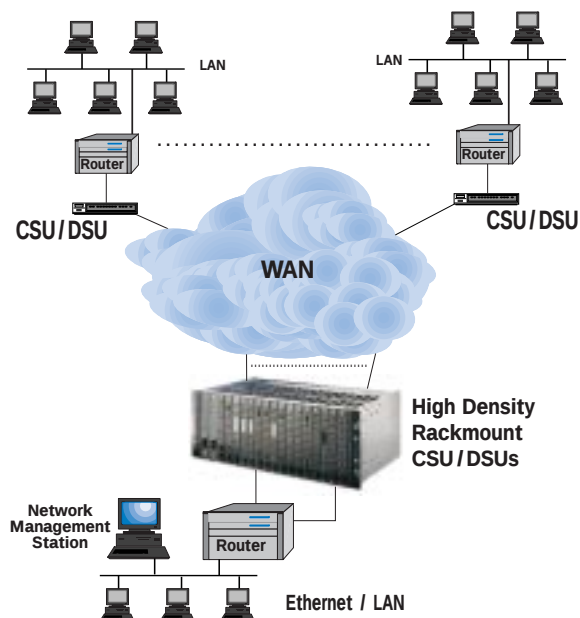
Figure 1 — Typical WAN Configuration with Standalone CSU/DSUs
