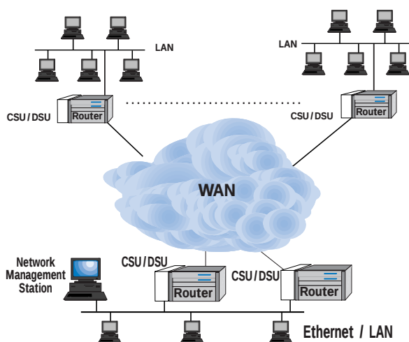
Figure 2 — WAN with Integrated Routers and Integrated CSU/DSUs
